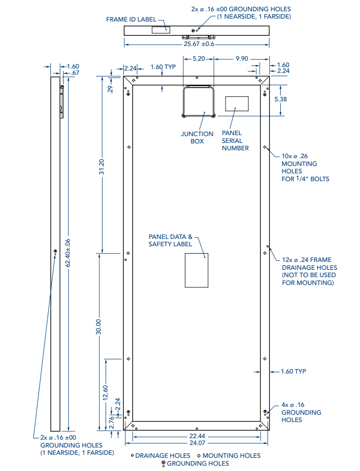
ALL DIMENSIONS IN INCHES; PANEL WEIGHT 27 LBS. (12.3 KG)
